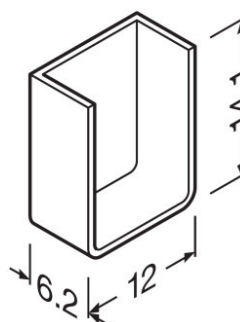
728404_Single sided endcaps for side-bending modules
