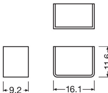
728403_Single sided endcaps for top-bending modules
